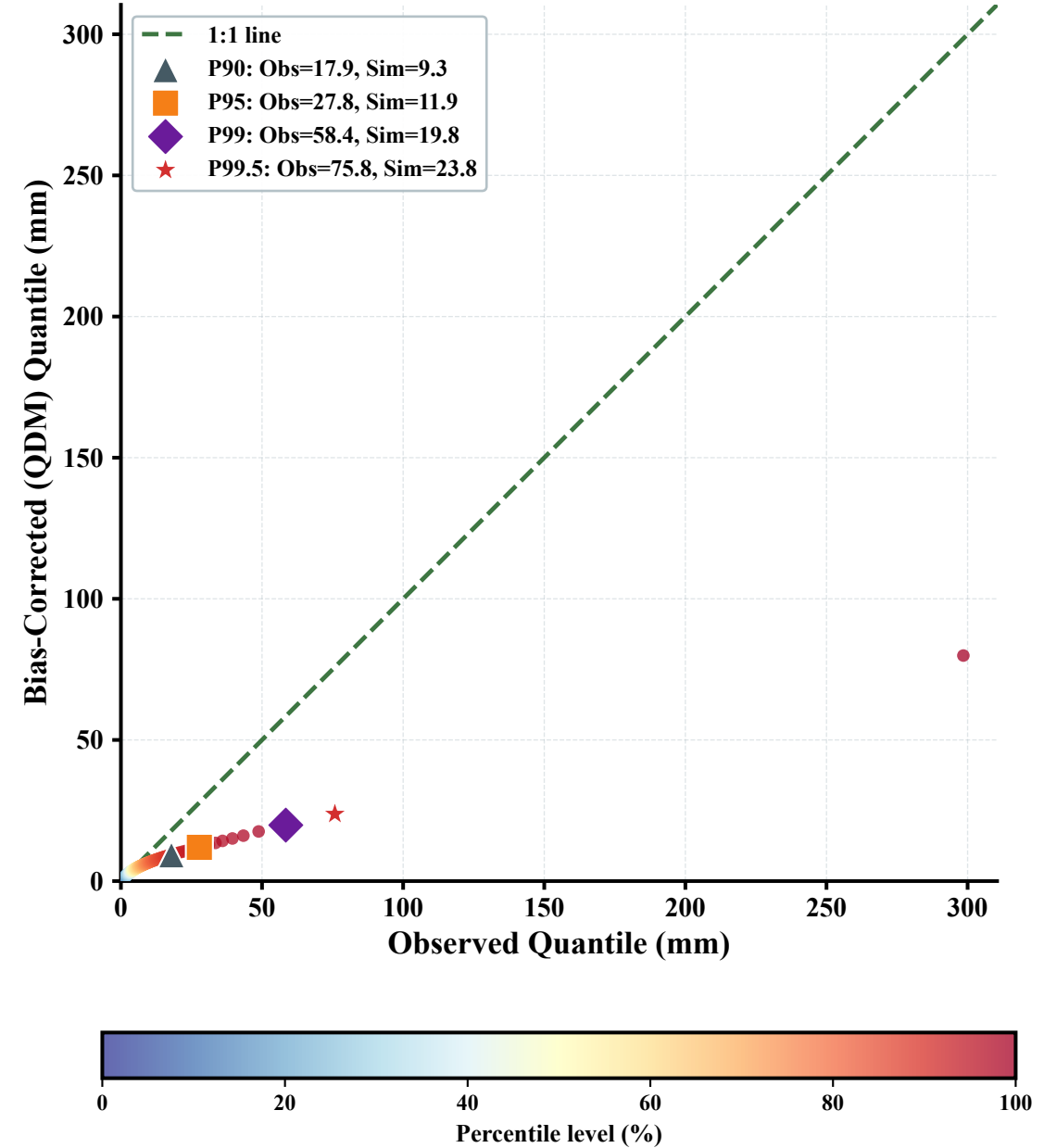
(b) Observed vs BC (QDM) QQ-RMSE = 17.02 mm
