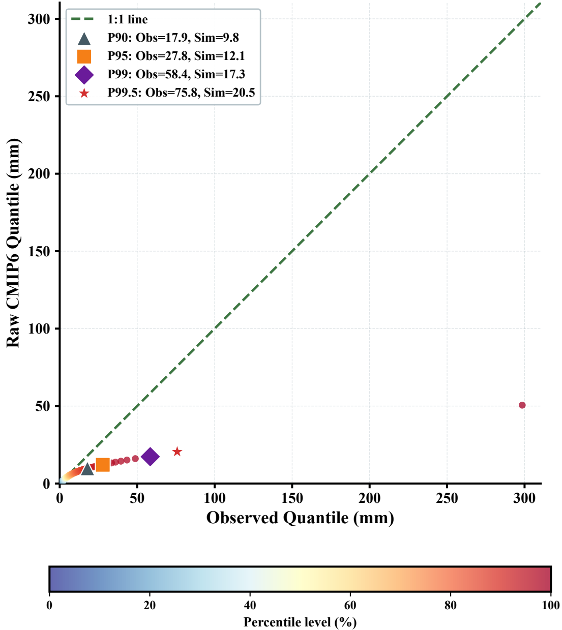
(a) Observed vs Raw CMIP6 QQ-RMSE = 18.98 mm
